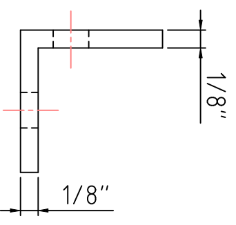
ALUMINUM AIR KNIFE COUPLING BRACKET
